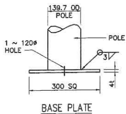
BASE PLATE
