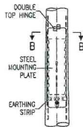
DETAIL OF FLUSH DOOR
