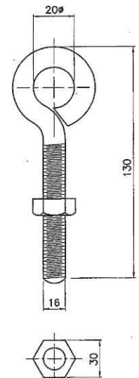
EYE BOLT
