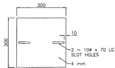
FLAT BASE PLATE
