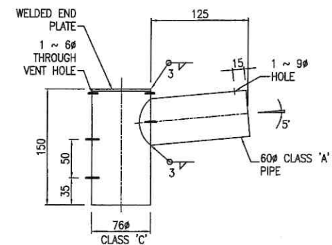
SPA - 125 SINGLE PIPE ADAPTOR
