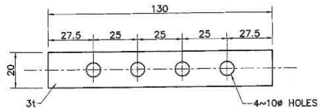
EARTHING STRIP
