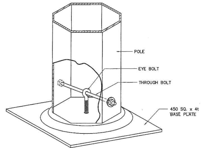
EYE BOLT
