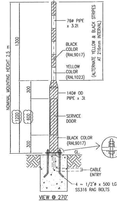
VIEW @ 270°
