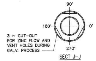
SECT J-J
