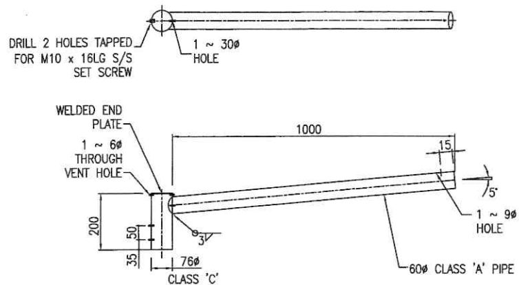
SPA - 1000 SINGLE PIPE ADAPTOR
