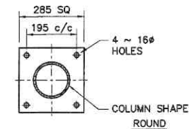
BASE FLANGE
