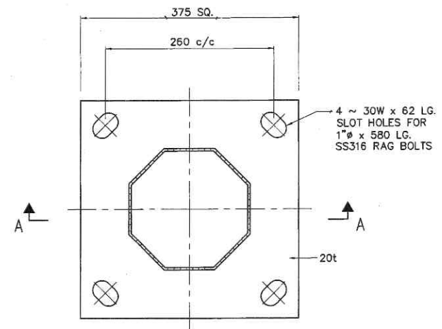
BASE FLANGE
