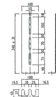
STEEL MOUNTING PLATE
