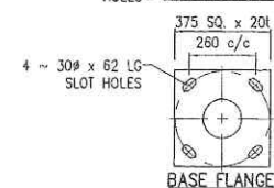
BASE FLANGE
