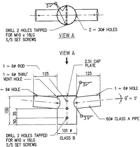
DPA - 125 DOUBLE PIPE ADAPTOR
