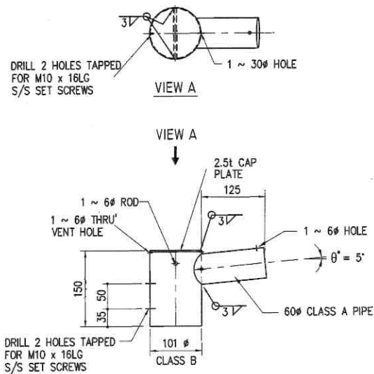
SPA - 125 SINGLE PIPE ADAPTOR
