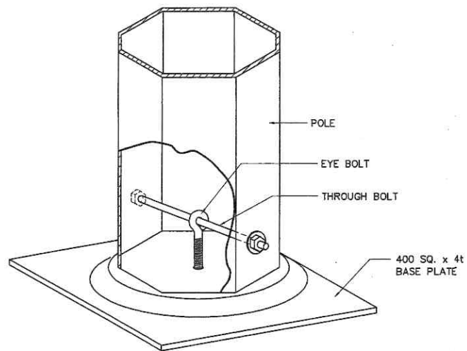
EYE BOLT
