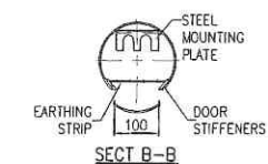
SECT B-B
