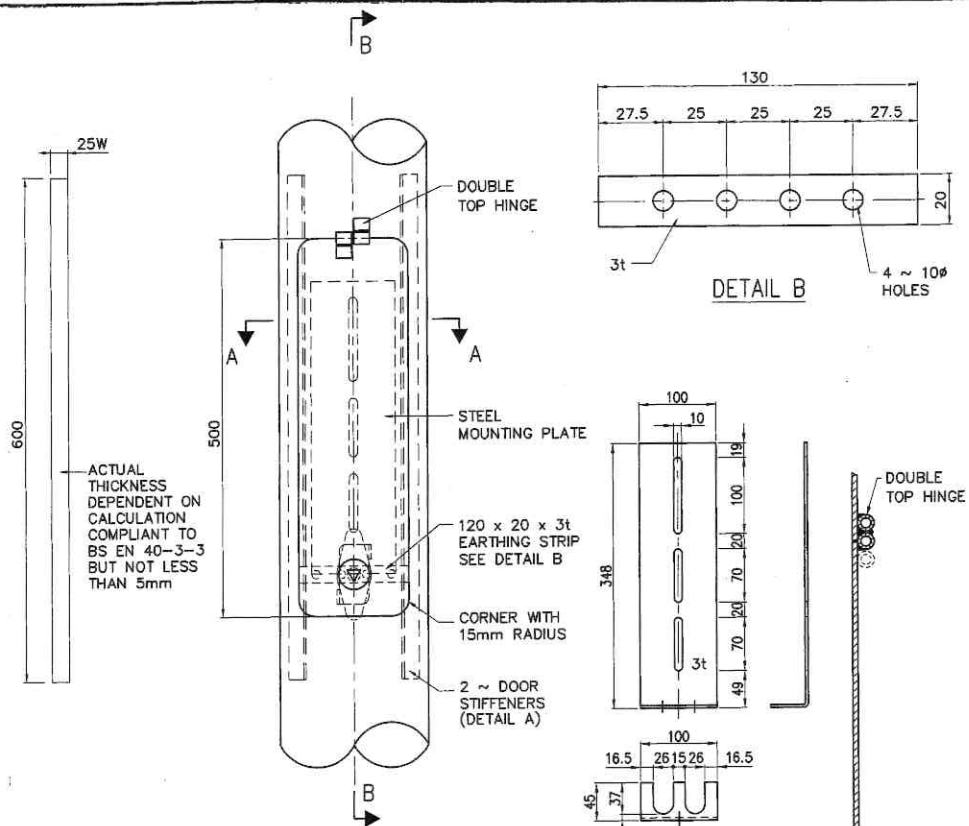
DETAIL OF FLUSHED DOOR
