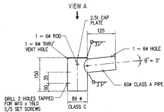
SPA - 125 SINGLE PIPE ADAPTOR
