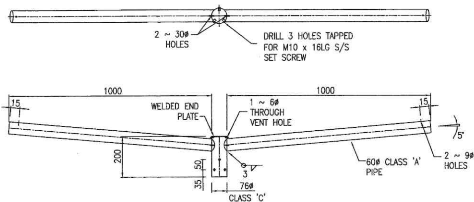
DPA - 1000 DOUBLE PIPE ADAPTOR
