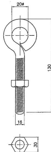
EYE BOLT
