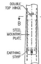
DETAIL OF FLUSH DOOR
