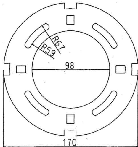
Bollard Baseplate Dimensions
