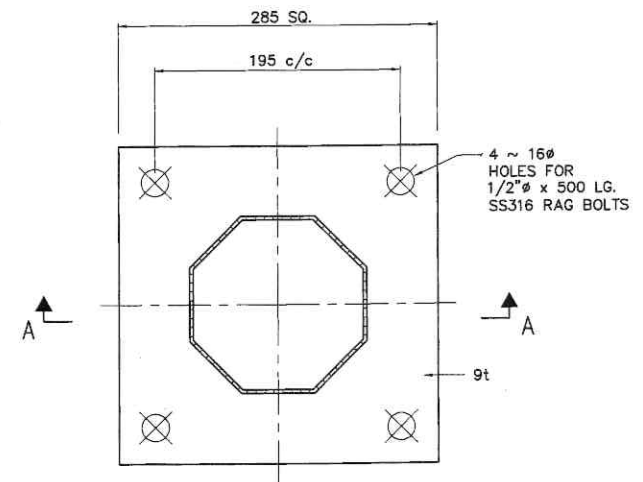
BASE FLANGE
