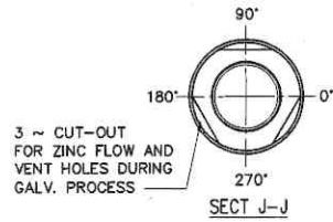
SECT J-J
