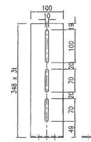
STEEL MOUNTING PLATE
