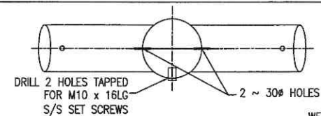
SPA - 125 SINGLE PIPE ADAPTOR
