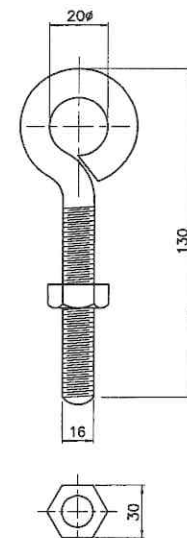
EYE BOLT
