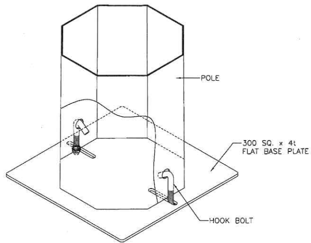
ISOMETRIC VIEW
