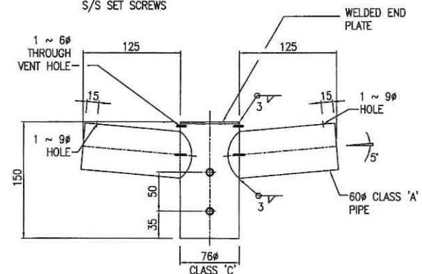
DPA - 125 DOUBLE PIPE ADAPTOR
