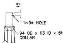
POLE TOP DETAILS
