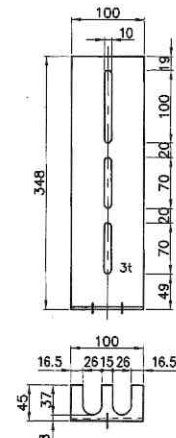
STEEL MOUNTING PLATE
