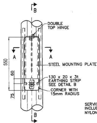
DETAIL OF FLUSHED DOOR
