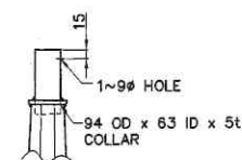
POLE TOP DETAILS
