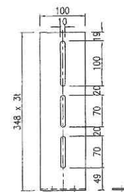
BASE SECTION
