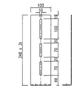
STEEL MOUNTING PLATE
