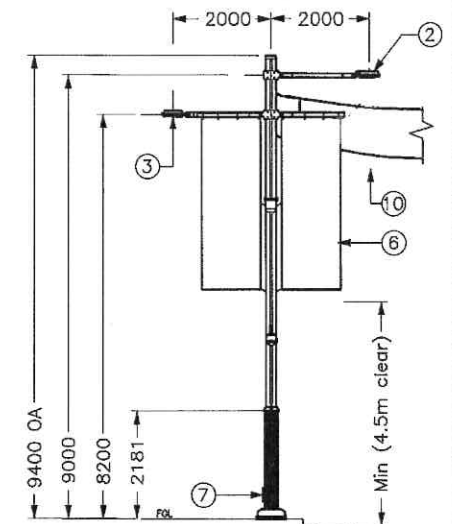
PARTIAL VIEW Cladding removed
