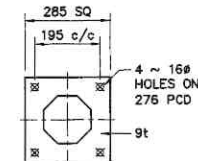
BASE FLANGE
