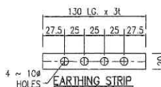
EARTHING STRIP
