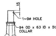
POLE TOP DETAILS
