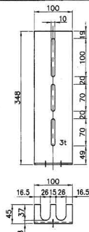
STEEL MOUNTING PLATE
