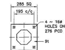
BASE FLANGE
