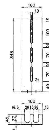
STEEL MOUNTING PLATE
