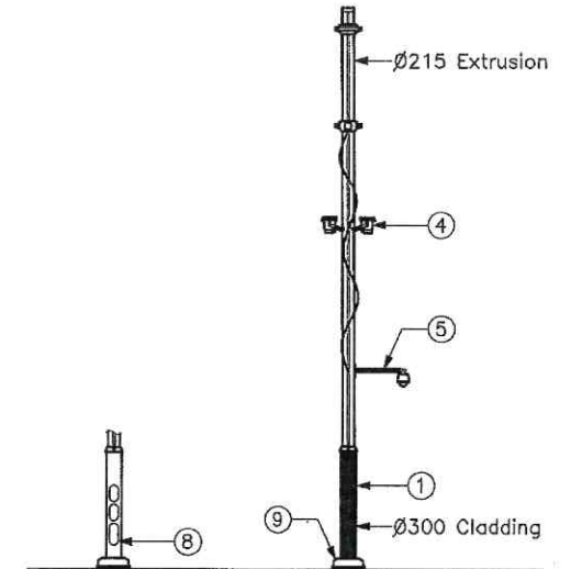
PARTIAL VIEW Cladding removed
