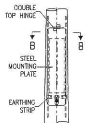
DETAIL OF FLUSH DOOR
